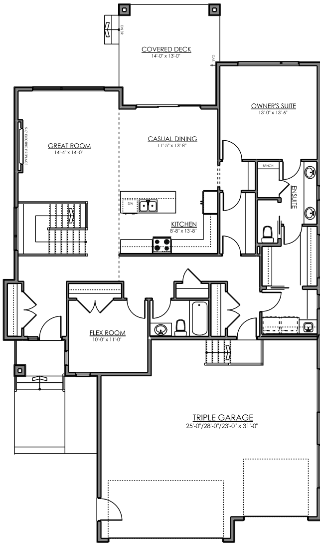
MAIN FLOOR PLAN - 1578 SQ.FT.
