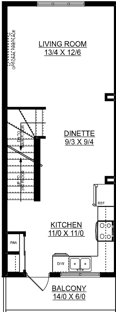
SECOND FLOOR PLAN 476 SQ. FT.
