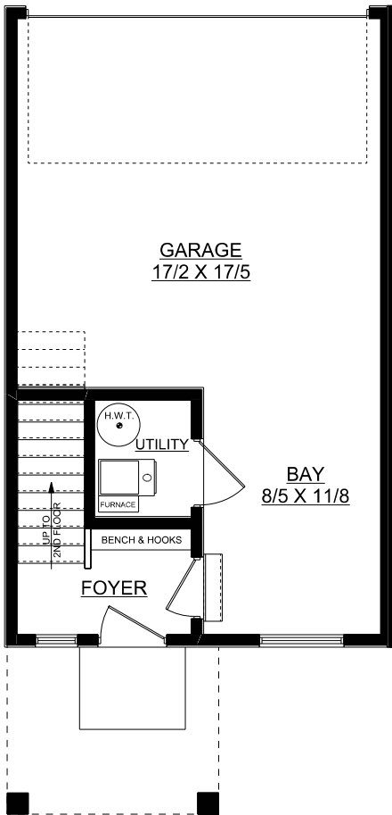
MAIN FLOOR PLAN 85 SQ. FT.
