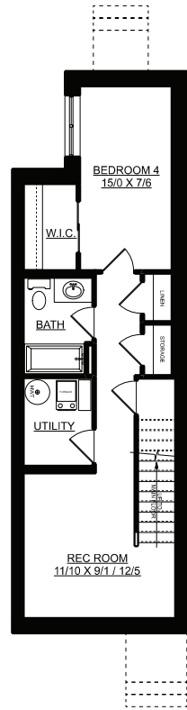
OPTIONAL BASEMENT PLAN 445 SQ. FT.
