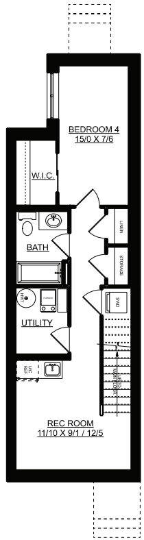
OPTIONAL BASEMENT W WET BAR & LAUNDRY 445 SQ. FT.
