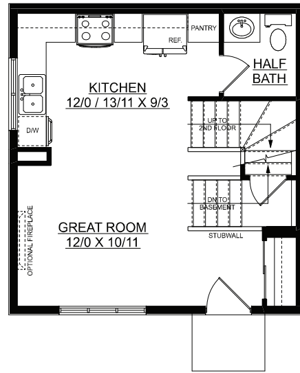
MAIN FLOOR PLAN 420 SQ.FT
