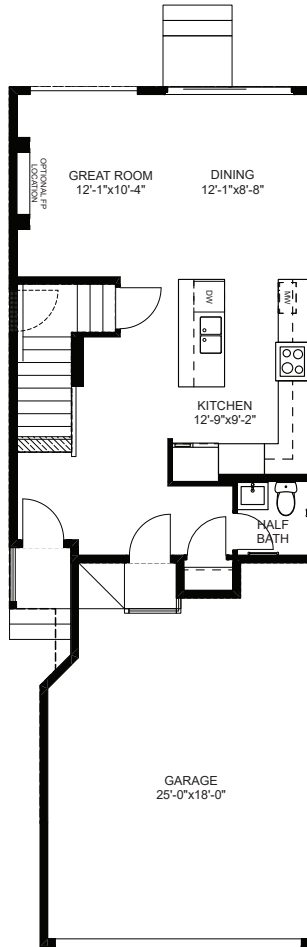
MAIN FLOOR PLAN 626 SQ. FT.
