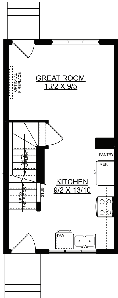
MAIN FLOOR PLAN 371 SQ.FT.
