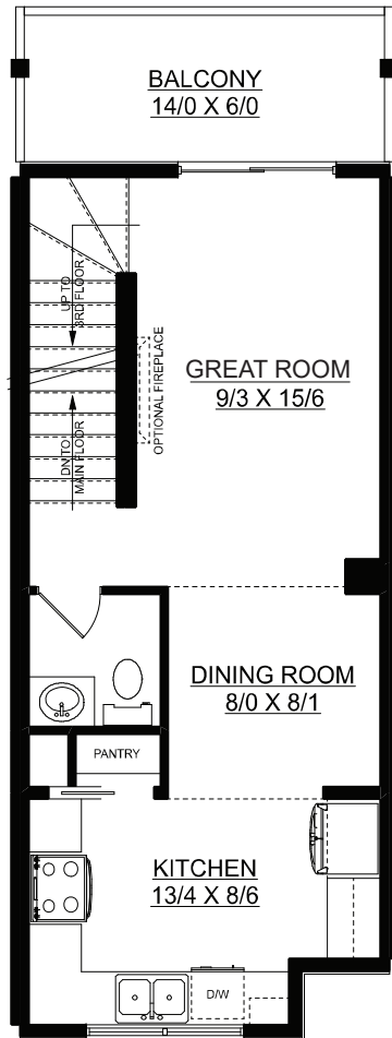
SECOND FLOOR PLAN 500 SQ.FT.
