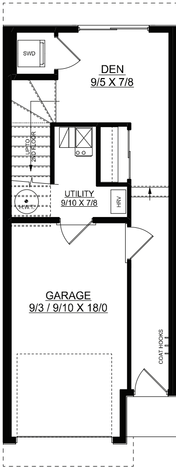
MAIN FLOOR PLAN 258 SQ.FT.
