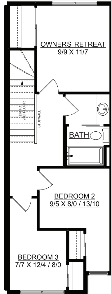
THIRD FLOOR PLAN 492 SQ.FT.
