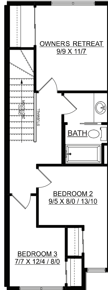
THIRD FLOOR PLAN 492 SQ.FT.
