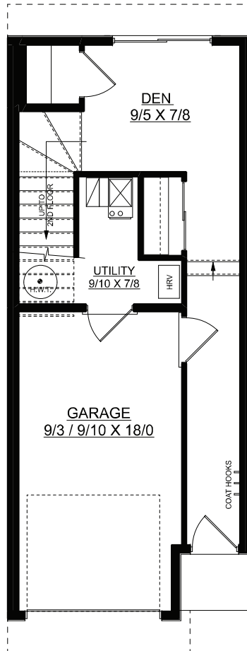
MAIN FLOOR PLAN 258 SQ.FT.
