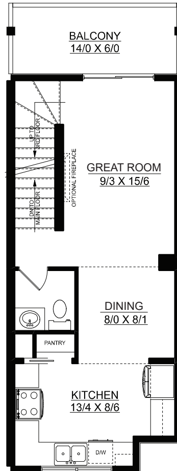
SECOND FLOOR PLAN 454 SQ.FT.
