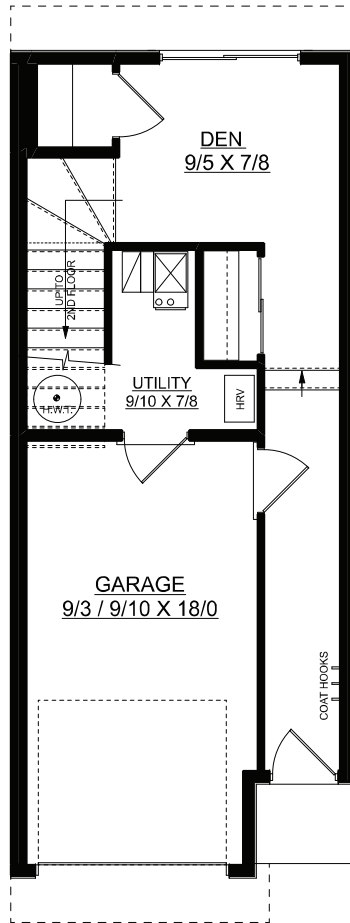
ENTRY PLAN 258 SQ.FT.
