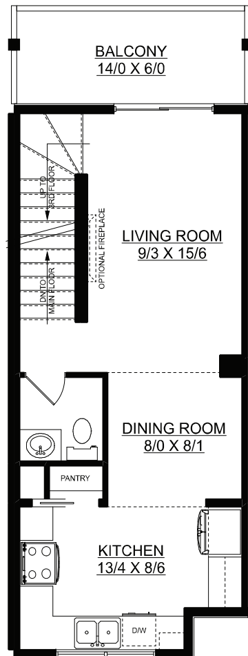
SECOND FLOOR PLAN 454 SQ.FT.
