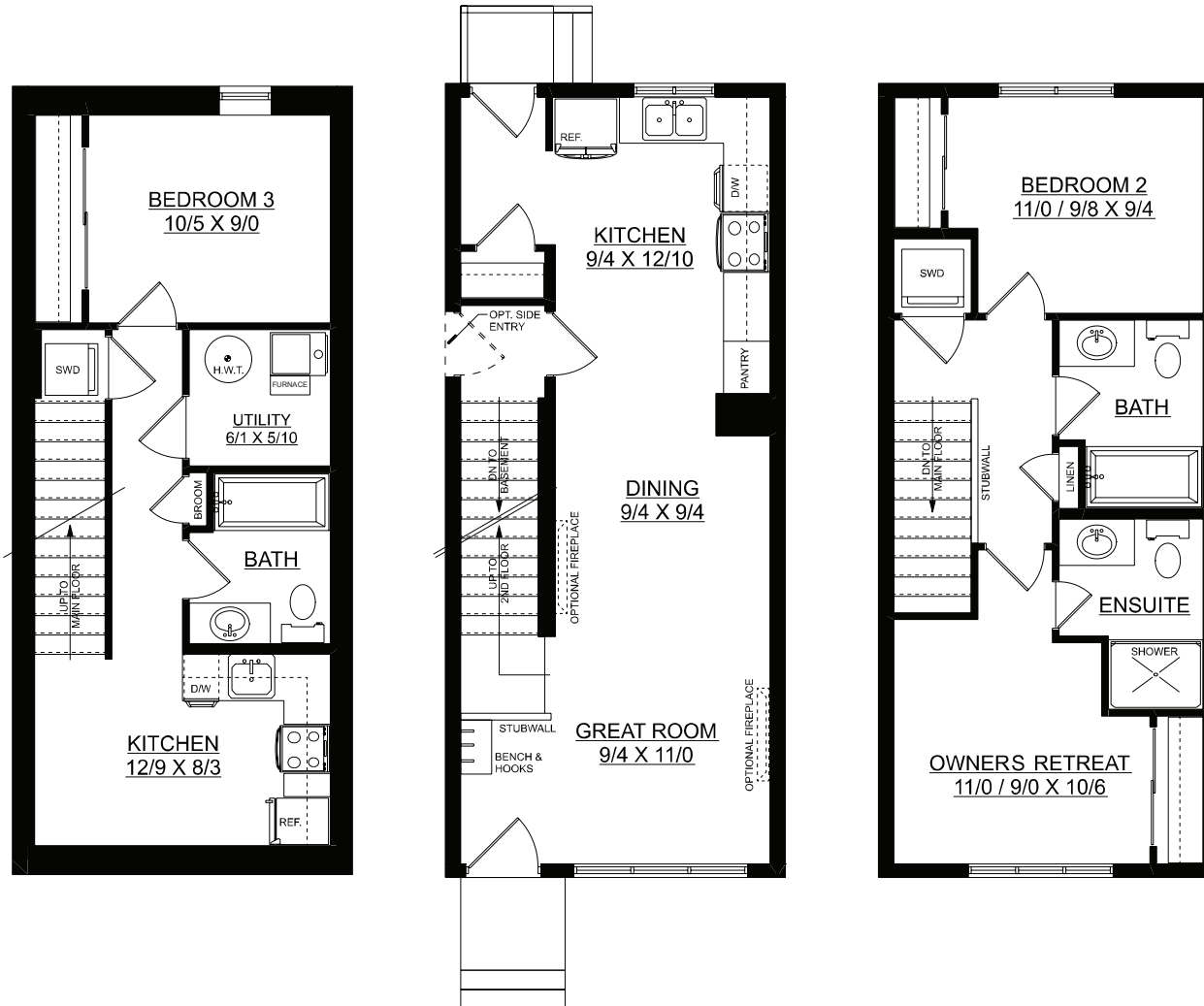
OPTIONAL BASEMENT SUITE 400 SQ. FT.
