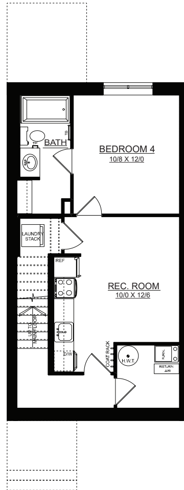
OPTIONAL BASEMENT PLAN 502 SQ. FT.
