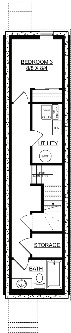
OPTIONAL BASEMENT PLAN 343 SQ. FT.
