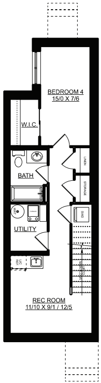
OPTIONAL BASEMENT W WET BAR & LAUNDRY 445 SQ. FT.
