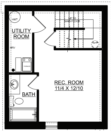
OPTIONAL BASEMENT PLAN W REC ROOM 308 SQ. FT.
