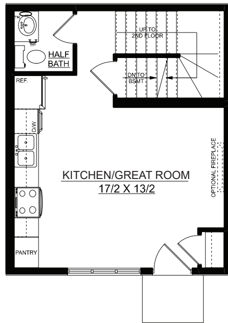
MAIN FLOOR PLAN 396 SQ. FT.
