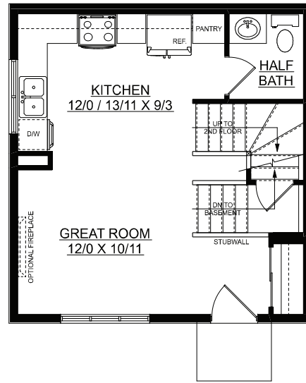
MAIN FLOOR PLAN 420 SQ.FT
