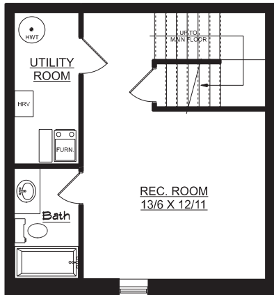
OPTIONAL BASEMENT PLAN W REC ROOM 348 SQ. FT.
