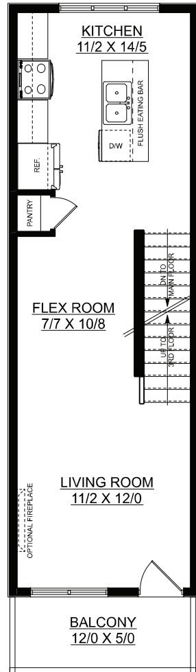
SECOND FLOOR PLAN 449 SQ. FT.
