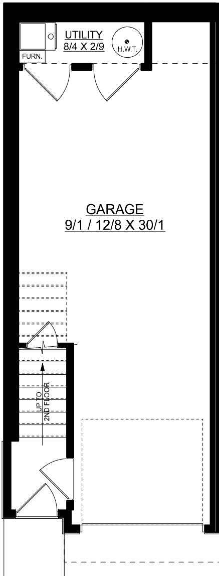
ENTRY PLAN 75 SQ.FT.
