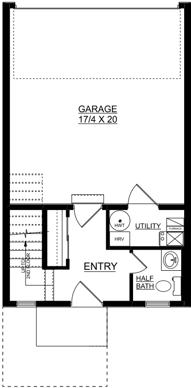
MAIN FLOOR PLAN 148 SQ. FT.
