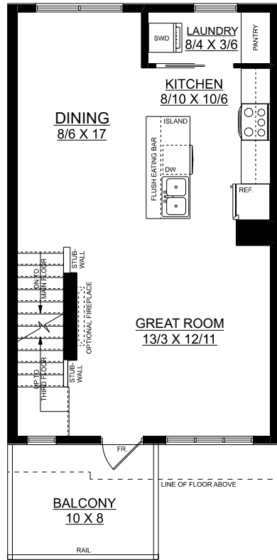
SECOND FLOOR PLAN 540 SQ. FT.
