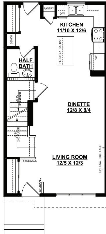
OPTIONAL BASEMENT PLAN 502 SQ. FT.
