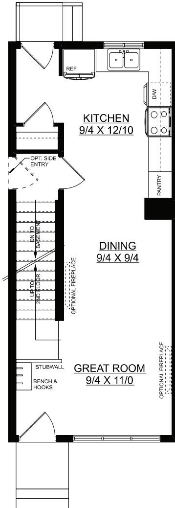
MAIN FLOOR PLAN 476 SQ. FT.
