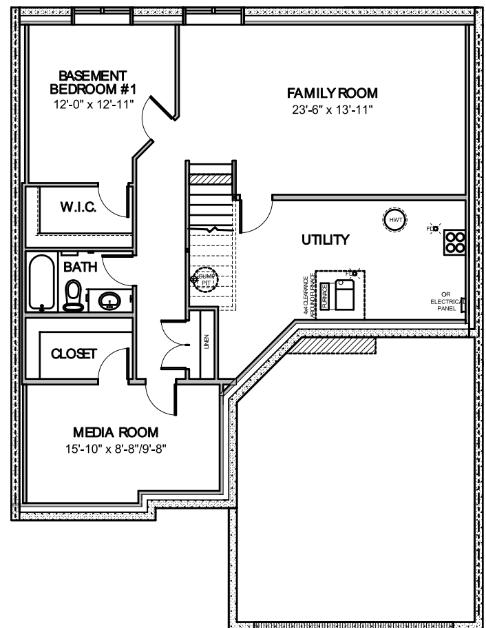
OPTIONAL BASEMENT DEVELOPMENT 871 SQ. FT.
