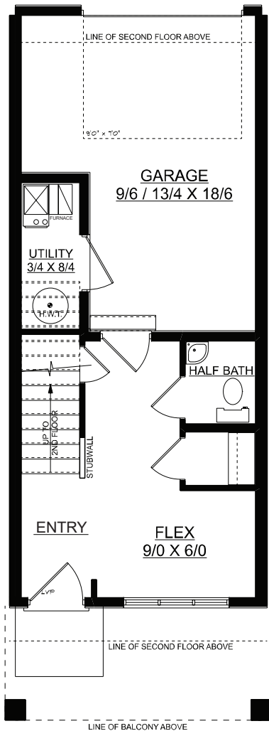
MAIN FLOOR PLAN 217 SQ.FT.
