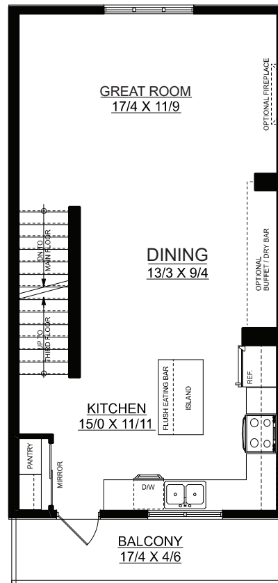
SECOND FLOOR PLAN 644 SQ. FT.
