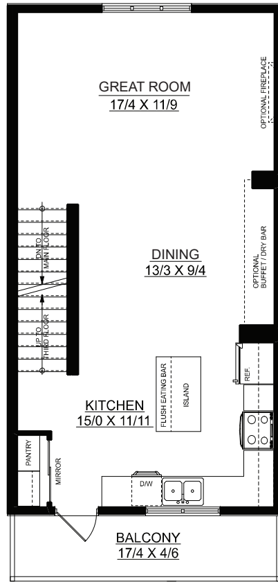
SECOND FLOOR PLAN 612 SQ. FT.
