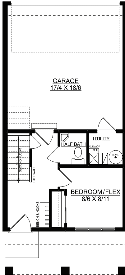
MAIN FLOOR PLAN 246 SQ. FT.
