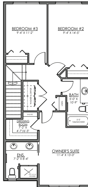
SECOND FLOOR PLAN 782 SQ. FT.
