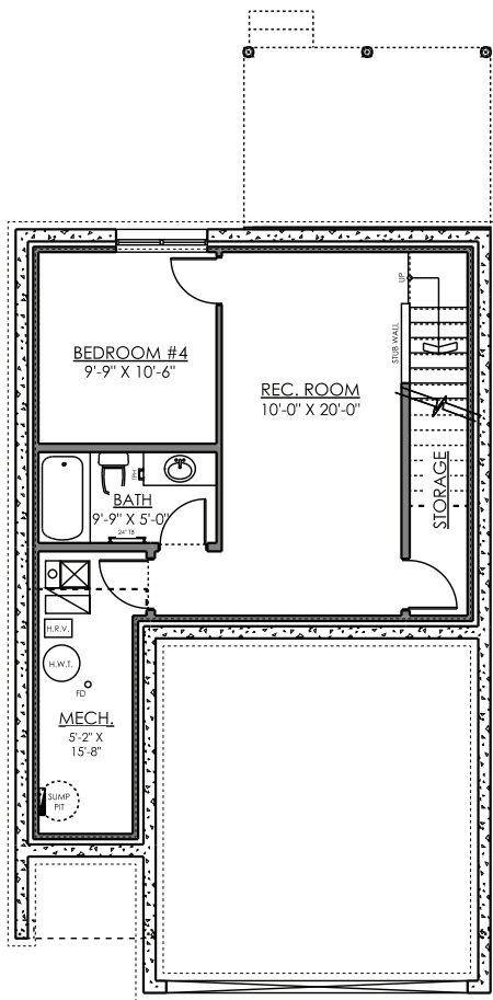
OPTIONAL BASEMENT PLAN 432 SQ. FT.
