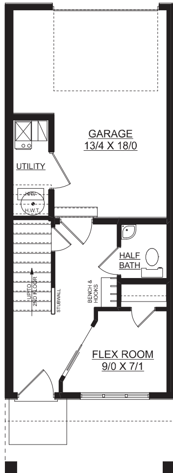
MAIN FLOOR PLAN 217 SQ. FT.
