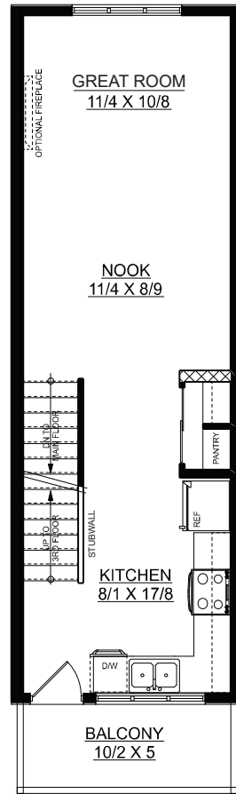
SECOND FLOOR PLAN 484 SQ. FT.
