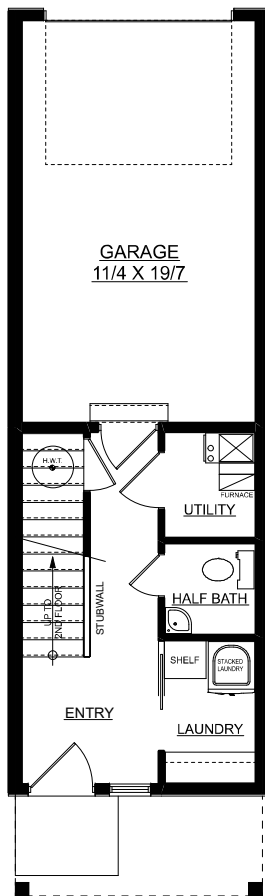
MAIN FLOOR PLAN 216 SQ. FT.
