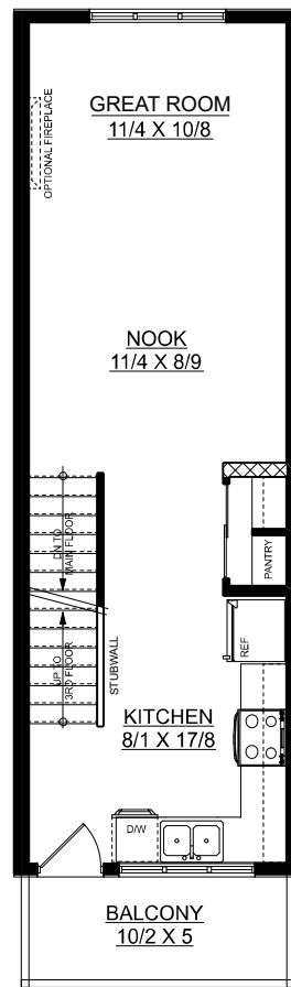
SECOND FLOOR PLAN 456 SQ. FT.
