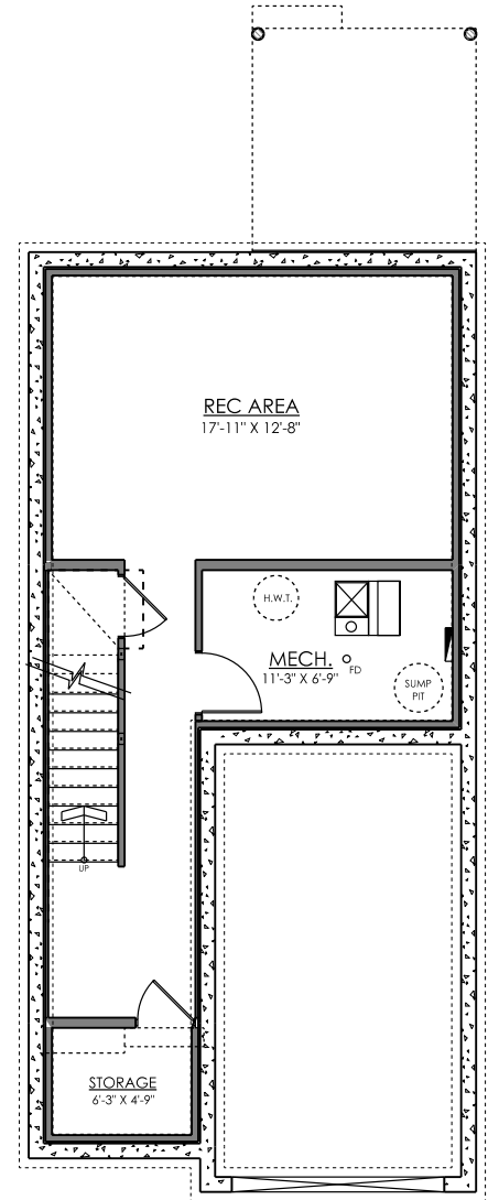
OPTIONAL BASEMENT PLAN 373 SQ. FT.
