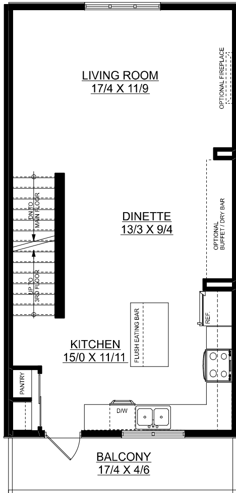
SECOND FLOOR PLAN 612 SQ. FT.
