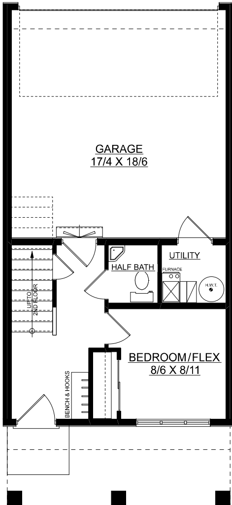
MAIN FLOOR PLAN 210 SQ. FT.
