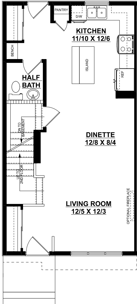
MAIN FLOOR PLAN 612 SQ. FT.
