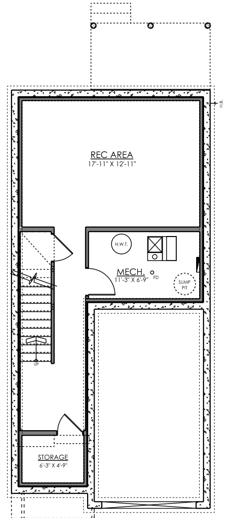
OPTIONAL BASEMENT PLAN 373 SQ. FT.
