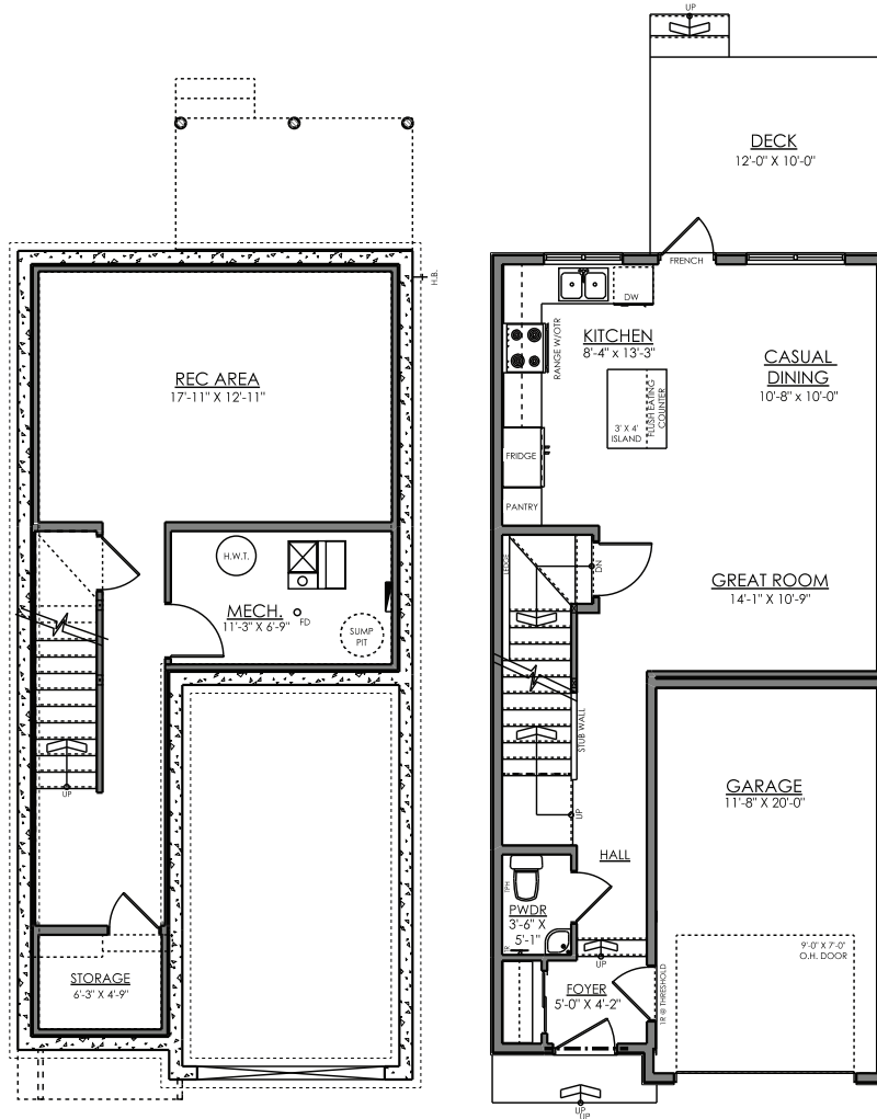
OPTIONAL BASEMENT PLAN 373 SQ. FT.
