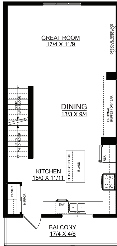
SECOND FLOOR PLAN 612 SQ. FT.
