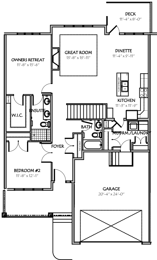
MAIN FLOOR PLAN 1384 SQ. FT.
